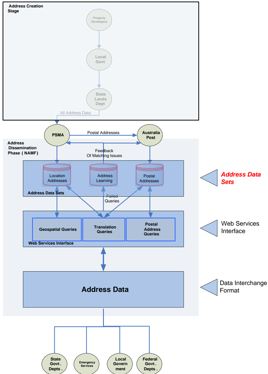
Figure 1: Address Data Supply Chain
